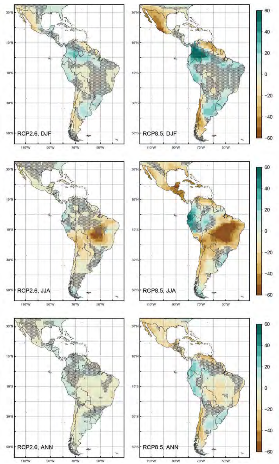
Figure 3.7: Multi-model mean of the percentage change in austral summer (DJF, top), winter (JJA, middle) and annual (bottom) precipitation for RCP2.6 (2°C world, left) and RCP8.5 (4°C world, right) for Latin America and the Caribbean by 2071–2099 relative to 1951–1980.
