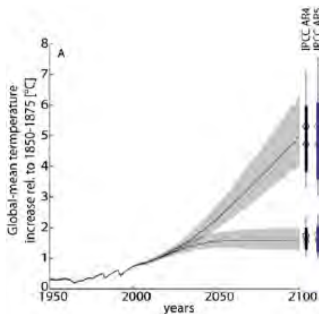
Figure 2.2: Climate-model projections of global-mean surface-air temperature for RCP2.6 (lower curves) and RCP8.5 (top curves).
