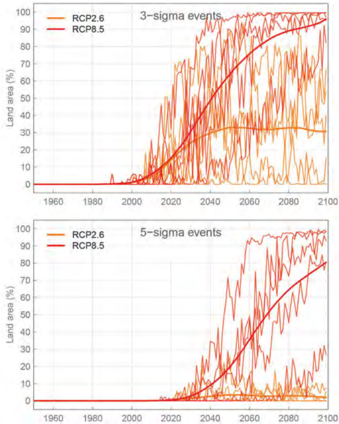
Figure 4.6: Multi-model mean (thick line) and individual models (thin lines) of the percentage of Middle East and North African land area warmer than 3-sigma (top) and 5-sigma (bottom) during boreal summer months (JJA) for scenarios RCP2.6 (2°C world) and RCP8.5 (4°C world).
