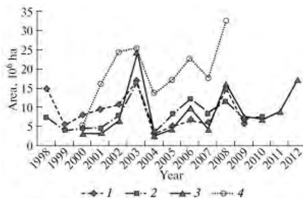
Figure 5.19: Dynamics of total area of wildfires in Russia's forests according to (1) GFDE3 (global fire emissions database); (2) refined data provided by the Institute of Forest, Russian Academy of Sciences; (3) Space Research Institute, Russian Academy of Sciences; and (4) Vivchar et al. (2010).
