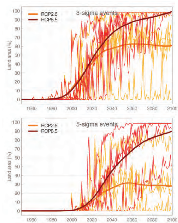
Figure 4.5: Multi-model mean (thick line) and individual models (thin lines) of the percentage of South East Asian land area warmer than 3-sigma (top) and 5-sigma during boreal summer months (JJA) for scenarios RCP2.6 and RCP8.5
